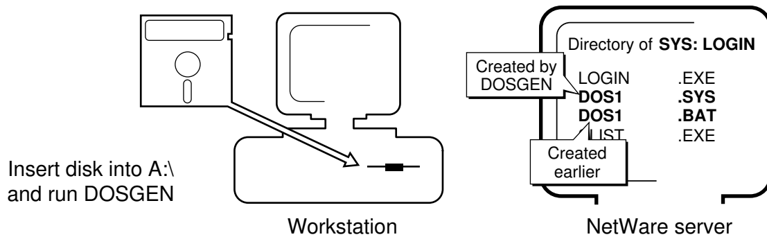
Figure 9-5 Run DOSGEN to create a .SYS file
